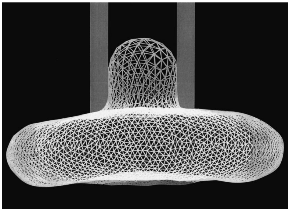
FIGURE 1 Simulation of a small erythrocyte under aspiration. The micropipette, indicated by the solid gray shading, has an inside diameter of 12s_R = 0.9 \mu\text{m} . The surface of the cell is triangulated with 6110 vertex nodes that represent the spectrin-actin junction complexes of the erythrocyte cytoskeleton. The volume of the cell is 0.6 times the fully inflated volume, and the simulation is drawn from the stress-free model in the free shape ensemble, as described in the text.
