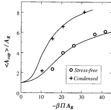
FIGURE 4 Ratio of the cap area per vertex \langle A_{\text{cap}} \rangle to the reference area per vertex A_R = \sqrt{3}s_R^2/2 in the free shape aspiration simulations of two effective models. The in-plane pressure \Pi in the aspiration simulations is found from the law of Laplace: \Pi = R_p P/2 . Shown for comparison by the solid curves are the area ratios expected for the same networks confined to two dimensions and subject to an in-plane stress (calculated in the mean field limit).
