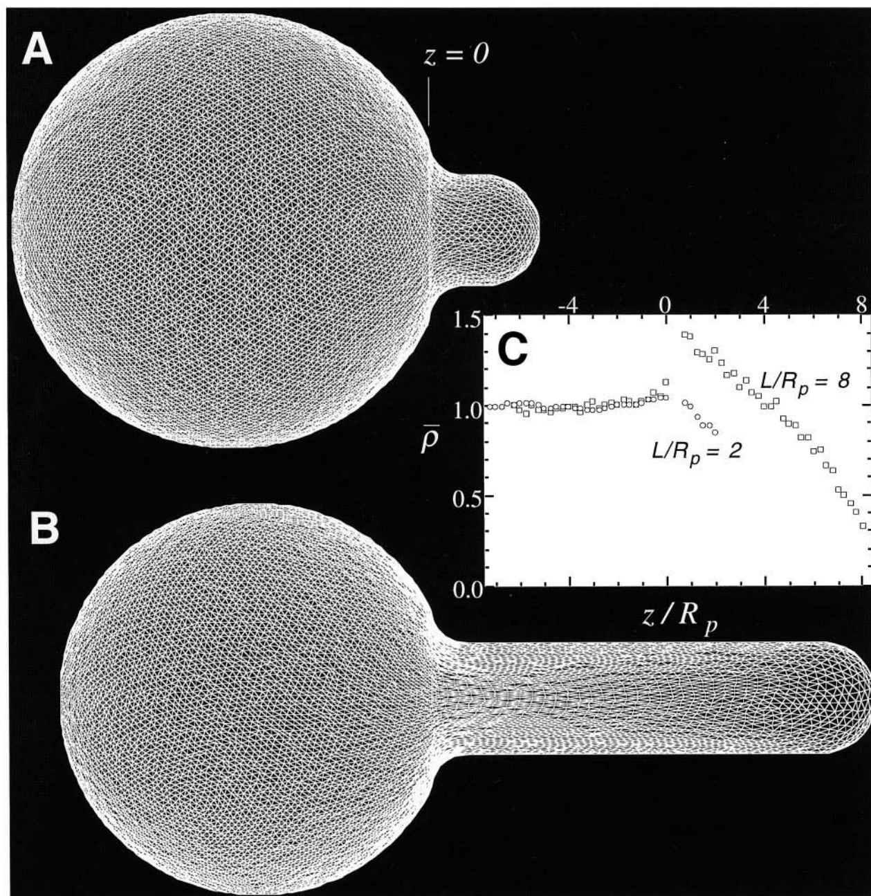
FIGURE 5 Simulations of an effective cytoskeletal network in two fixed shape ensembles of different aspiration lengths ( A and B ); also shown ( C ) are the corresponding relative density profiles. The network consists of 18,434 nodes, predominantly sixfold coordinated, and the nodes are confined in their motions to four smoothly connected and well-defined surfaces: a large spherical body, a right circular cylinder of radius R_p , a quarter-sector of a torus (minor radius 0.6R_p ) that connects the cylinder and sphere, and a hemispherical cap. The latter three surfaces define the aspirated projection, of length L , from z = 0 . The projection is formed incrementally through a sequence of equi-area transformations from an initial sphere of radius R_s . In physical units, if s_R = 75 nm is assumed, then R_p = 668 nm and the initial R_s = 2.67 \mu m. The density profiles, as projected into bins along the z axis, are normalized in C by the homogeneous density of a network on a sphere. The particular model shown is the prestress model.
